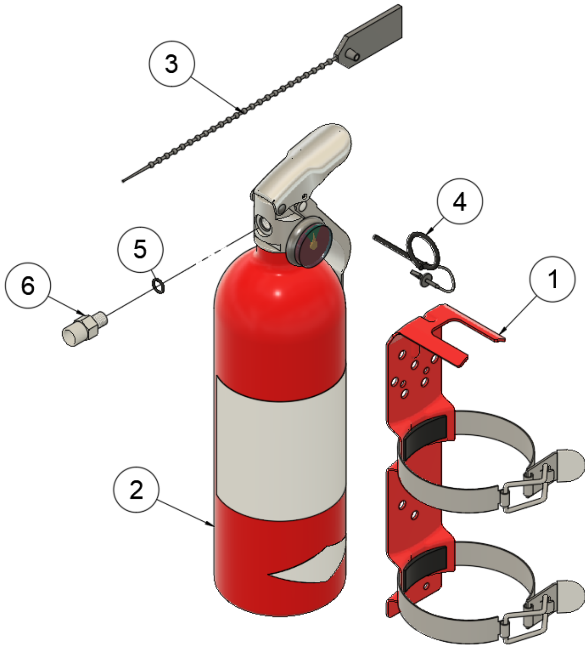
Figure 7. 355N69953TS Fire Extinguisher Assembly
