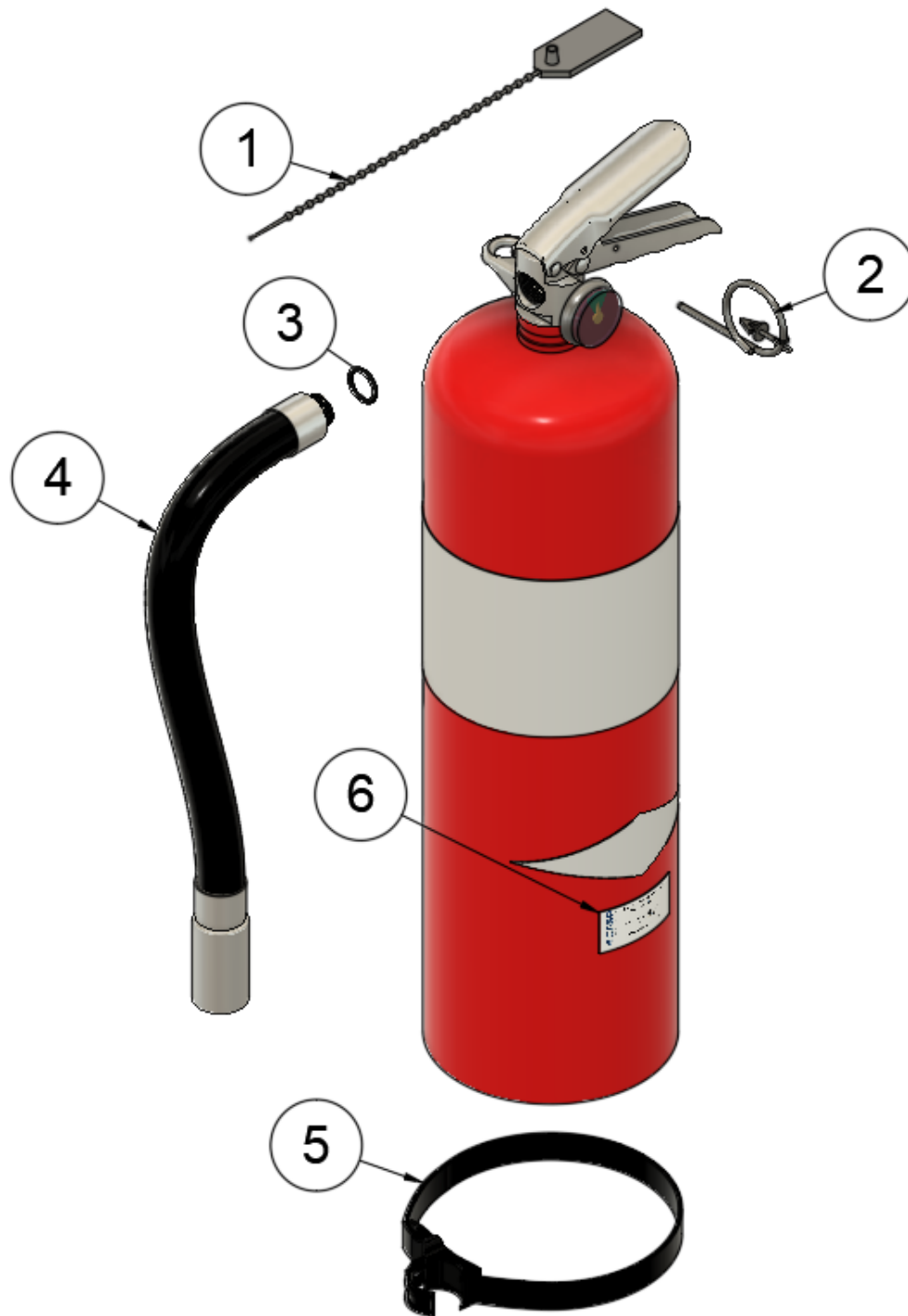
Figure 5. 125H673 Fire Extinguisher Assembly
