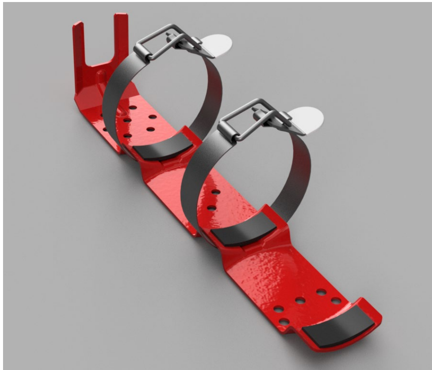
Figure 3. 25261 Bracket Assembly Model 898
